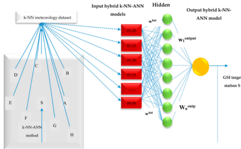
10 Figure 4. The proposed forecasting model using a k -nearest neighbor and artificial neural network ( k -NN-ANN) model.
