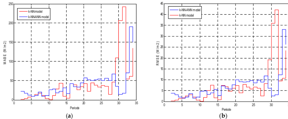
Figure 11. (a) MABE coefficients between actual data and GSI forecasts using the k -NN-ANN model on the test data set; and (b) RMSE coefficients between actual data and GSI forecasts using the k -NN-ANN model on the test data set.
